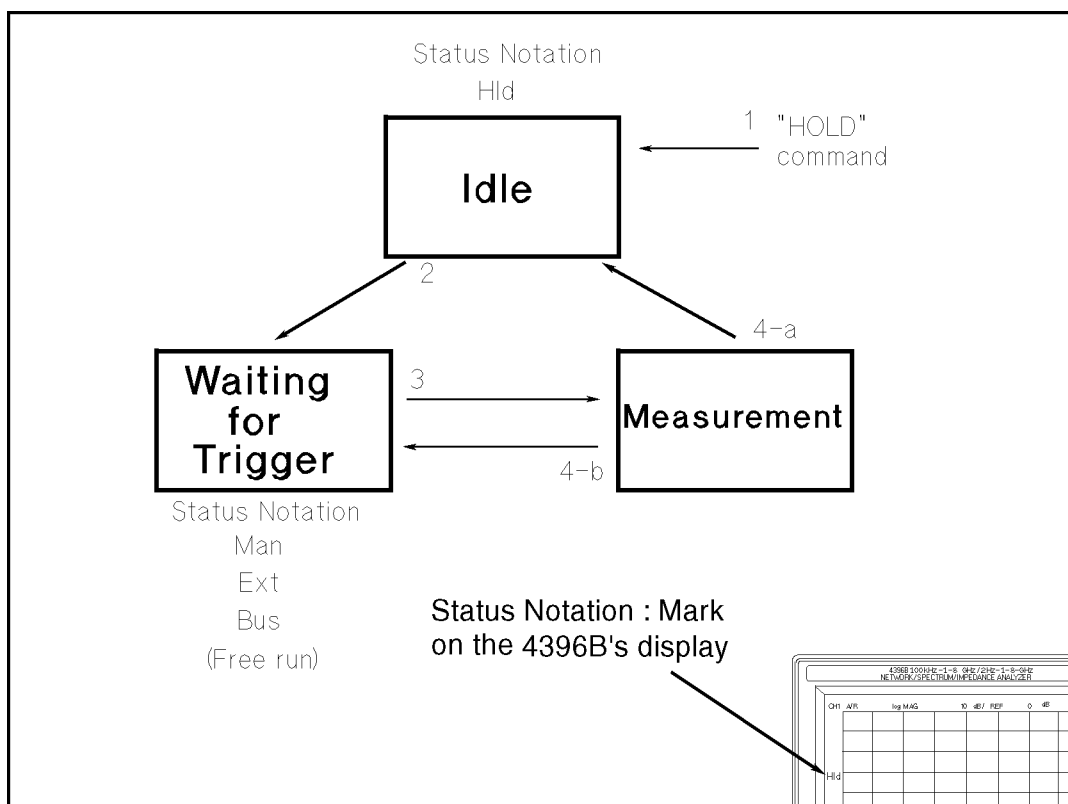
Figure 2-1. Trigger System
