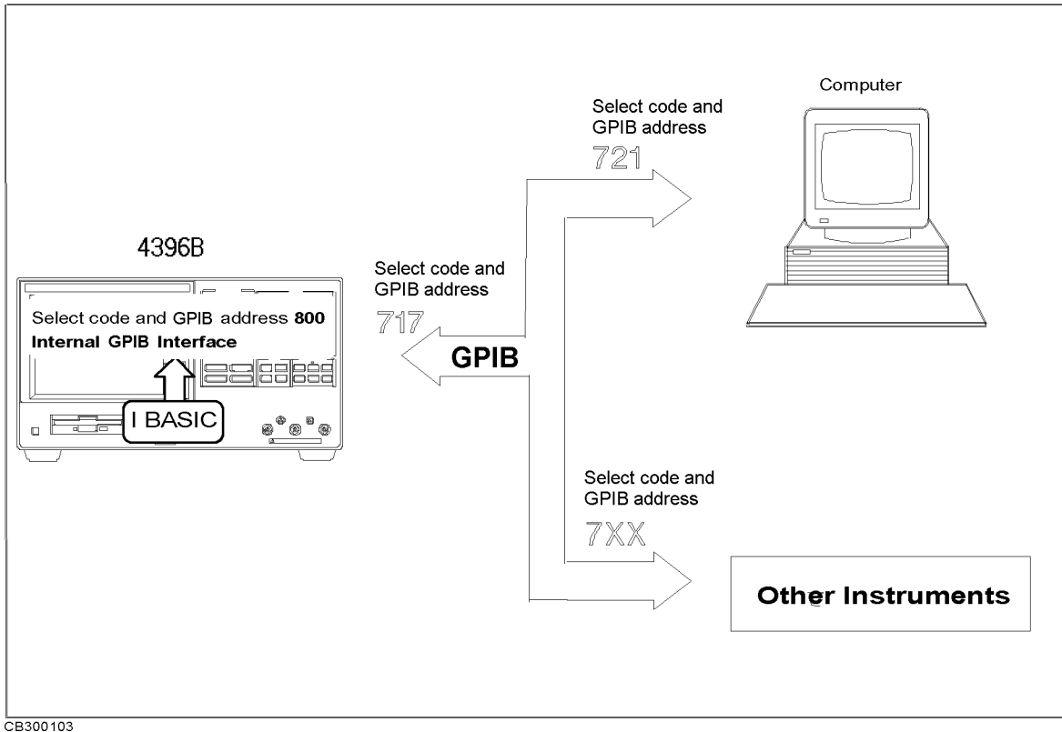
Figure 2-1. Configuration Example of the HP Instrument BASIC System
